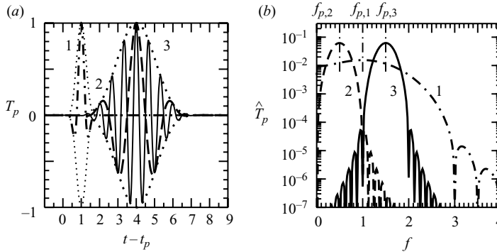
FIGURE 3. Time functions for three pulse disturbances. (a) Pulse disturbances versus time. (b) Frequency spectra for the pulse disturbances. Pulse type 1: short duration pulse ( -\cdot- ); pulse type 2: low-frequency pulse ( - - - ); pulse type 3: high-frequency pulse ( - ). Note, a sampling period of \Delta t = 40 is used for computing the spectra from the time functions.
